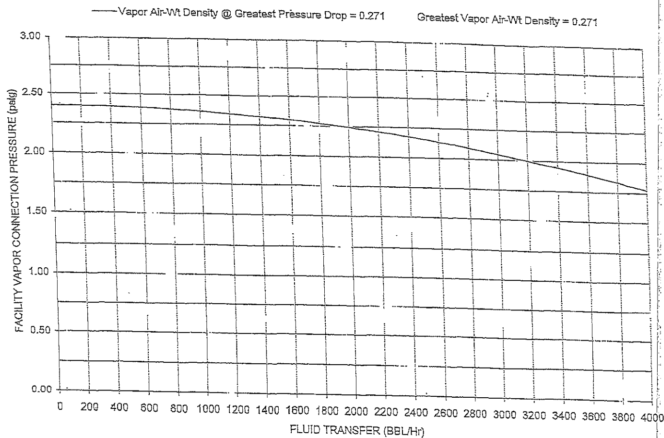
FIG. 2 - FLUID TRANSFER vs FACILITY VAPOR CONNECTION PRESSURE
