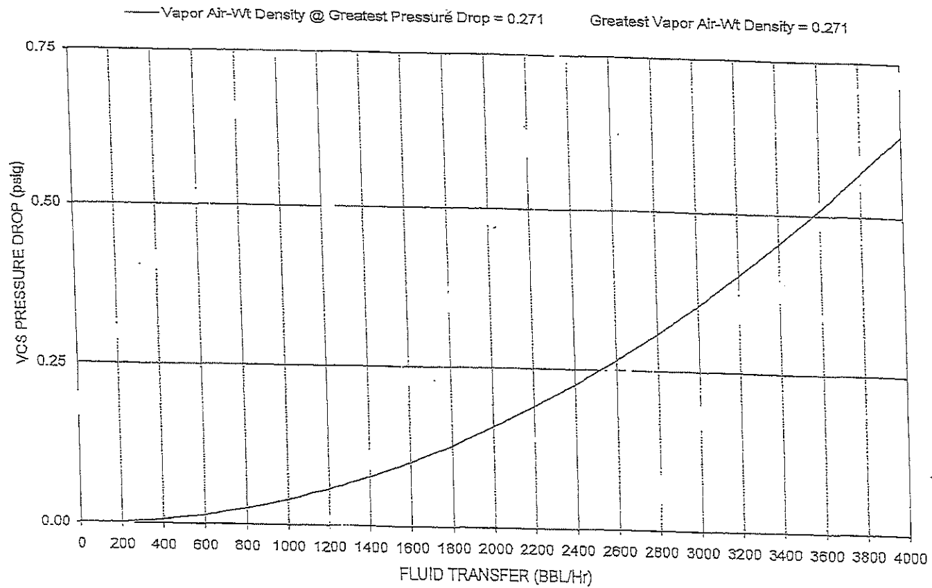
FIG. 1 - FLUID TRANSFER vs VCS PRESSURE DROP
